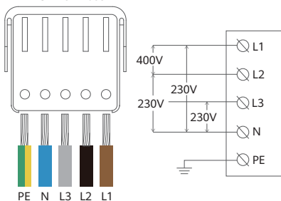
TN&TT 3-Phasen
