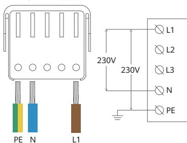
TN&TT 3-Phasen
