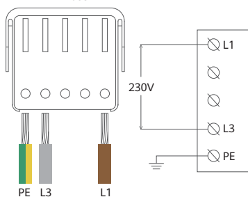
IT 1-Phasen
